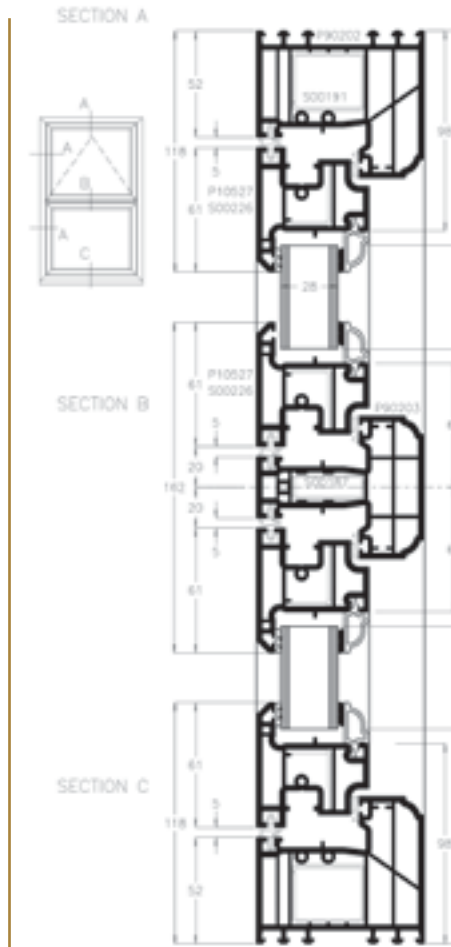
Flush 72mm outer frame (large)
