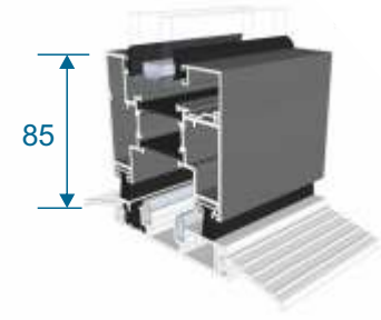
(F) 15mm Threshold
