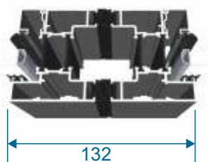
(C) Meeting Stile
